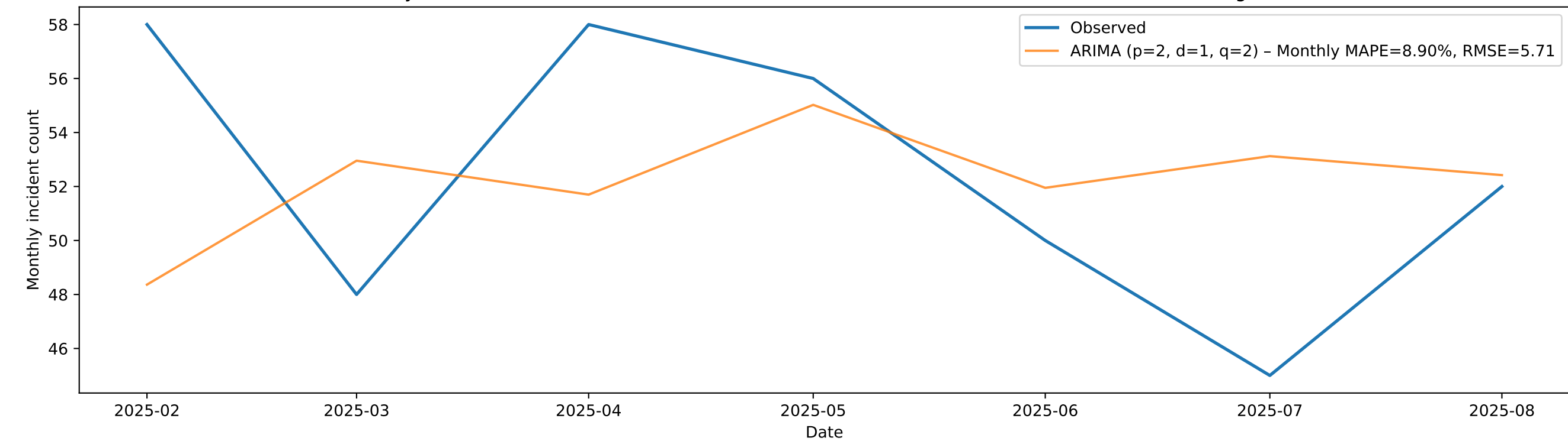
Monthly Traffic Incidents in Anadolu Street: Best Time-series Model vs Observed (Feb 2025-Aug 2025)
